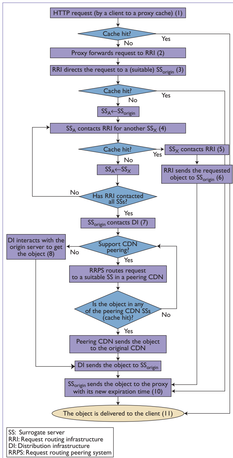
Figure 1. Delivering the requested object to the client. "Cache hit" indicates that the cache contains a current version of the object.
