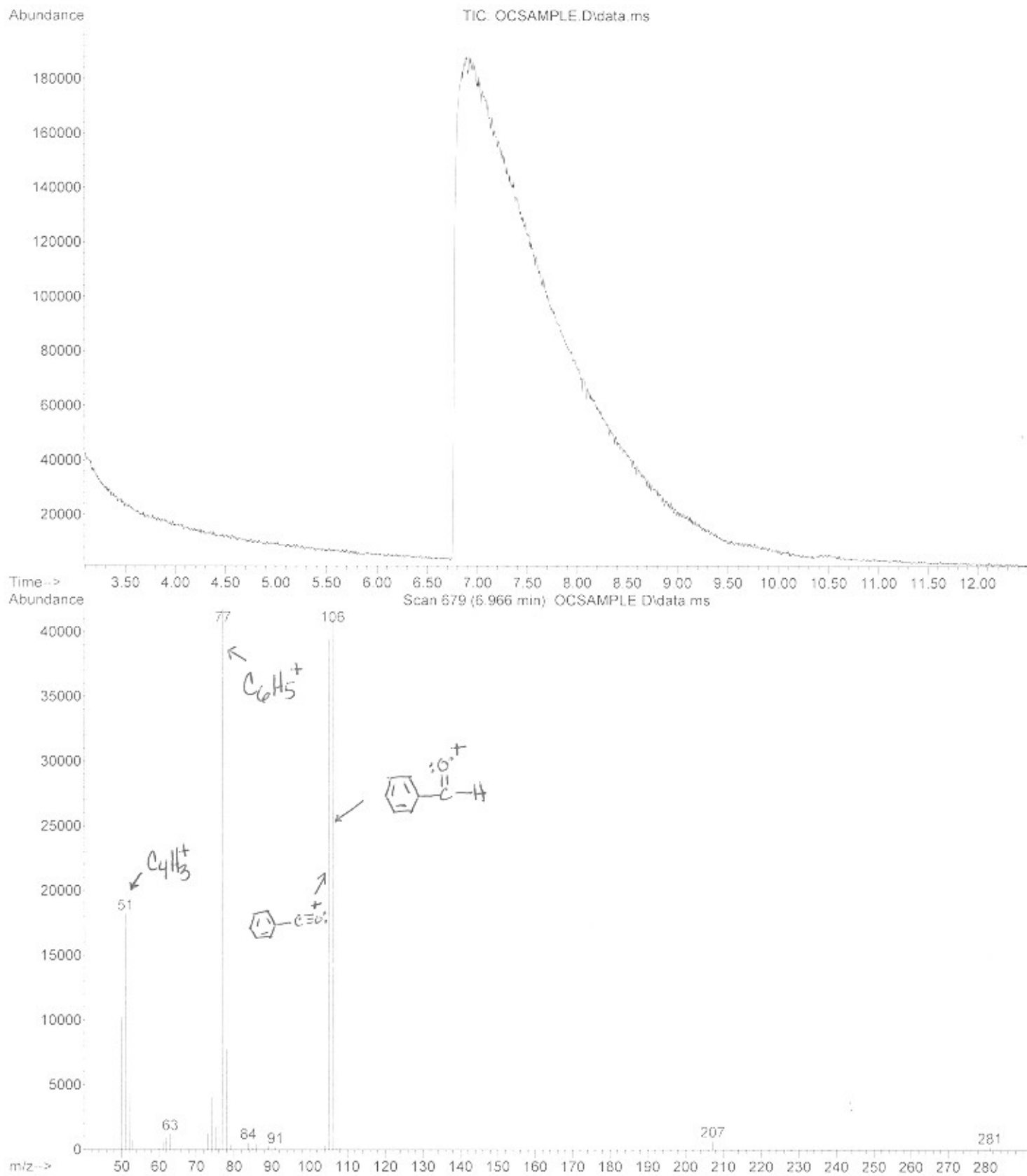
Figure 2. Gas chromatogram/mass Spectrum of benzaldehyde in CH 2 Cl 2 .
